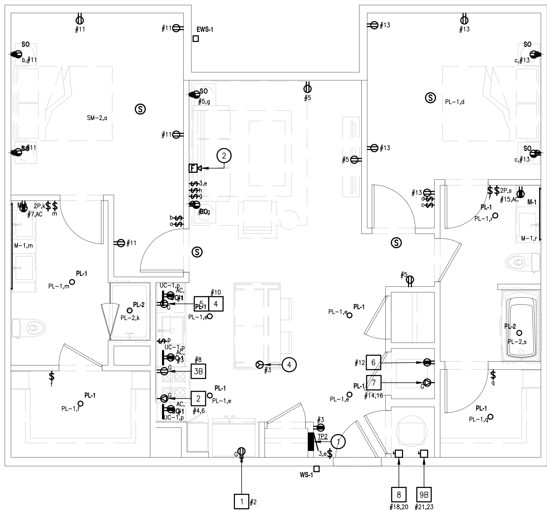
4 BUILDING 2 UNIT TYPE B2 ELECTRICAL PLAN A3.02B SCALE: 1/4" = 1'-0"
